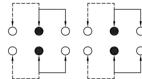
SCHMATIC (NON-SHORTING)
